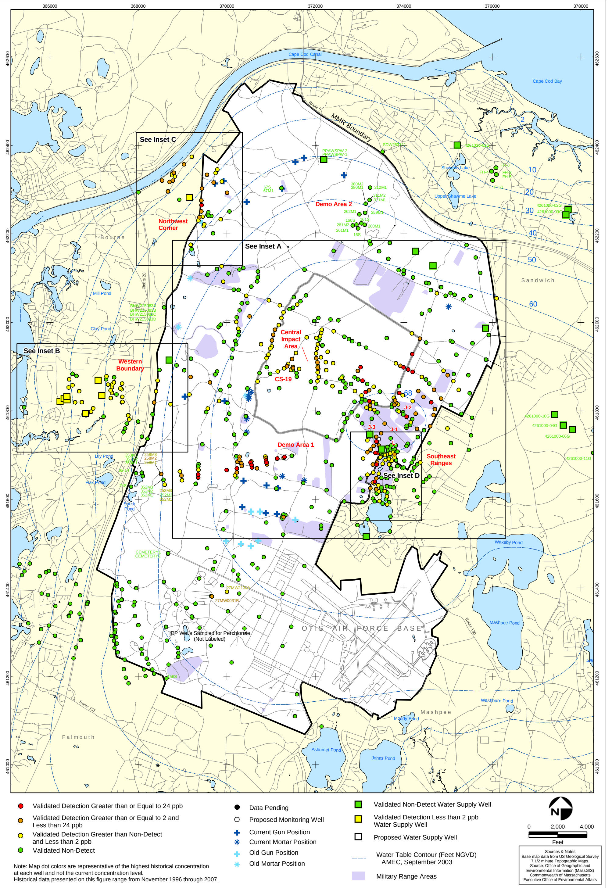
Perchlorate in Groundwater Compared to a 2 ppb Concentration Validated Data as of 11/28/07
