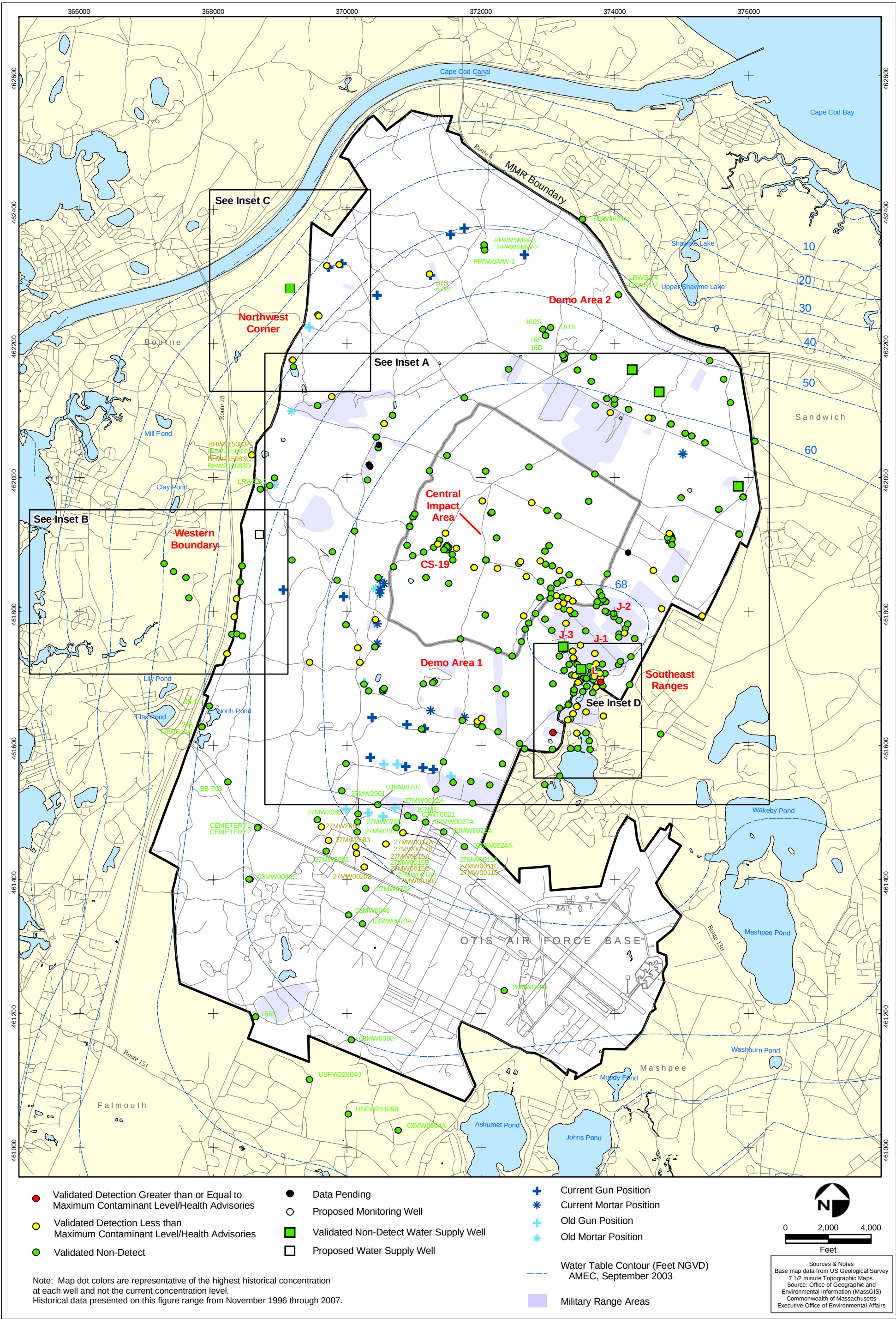
Semi-Volatile Organic Compounds (Excluding BEHP) in Groundwater Compared to Maximum Contaminant Level/Health Advisories Validated Data as of 9/26/07 AMEC Earth & Environmental, Inc. Westford, Massachusetts FIGURE 5
