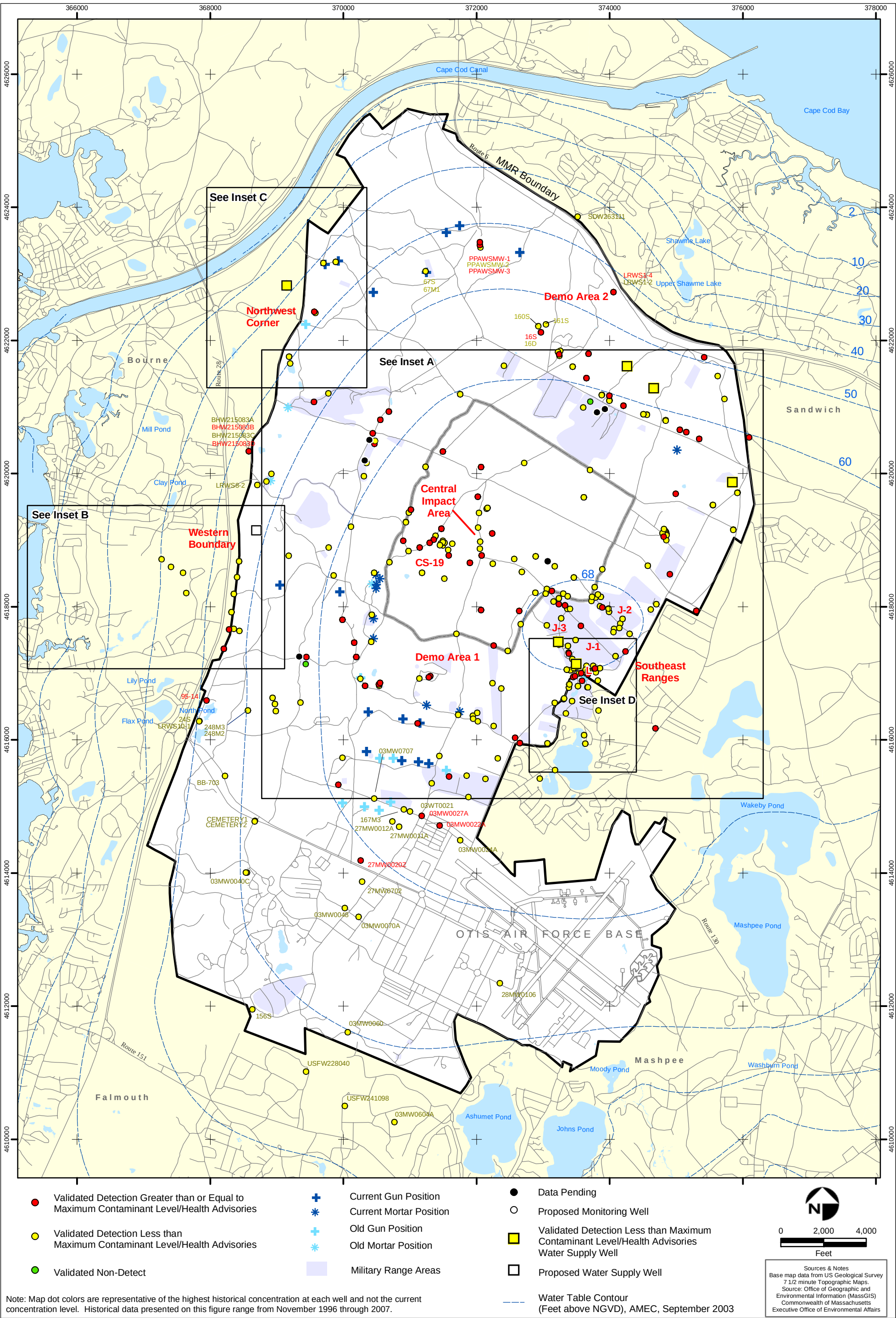
AMEC Earth & Environmental, Inc. Westford, Massachusetts Metals in Groundwater Compared to Maximum Contaminant Level/Health Advisories Validated Data as of 9/26/07 FIGURE 2
