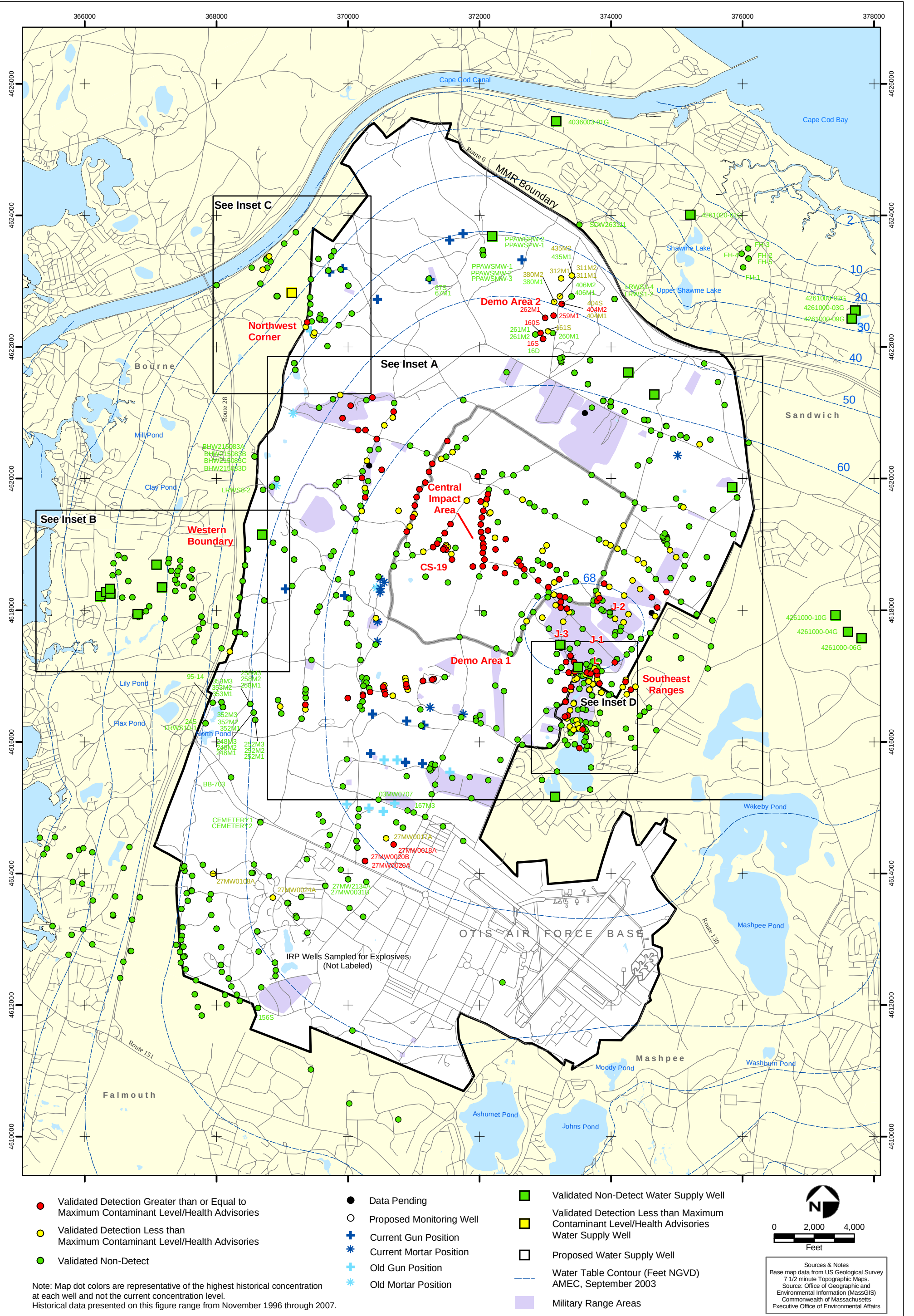
Explosives in Groundwater Compared to Maximum Contaminant Level/Health Advisories Validated Data as of 11/28/07
