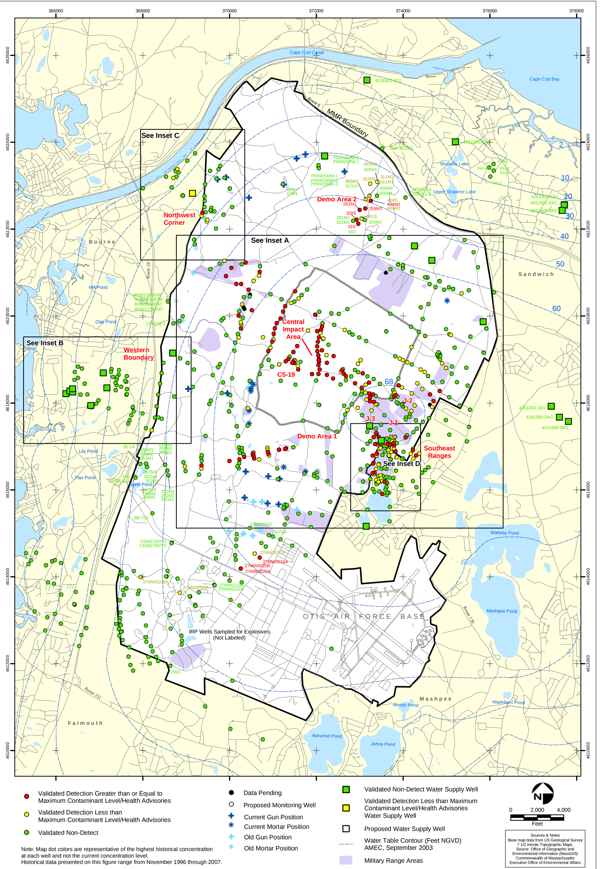
Explosives in Groundwater Compared to Maximum Contaminant Level/Health Advisories Validated Data as of 8/31/07
