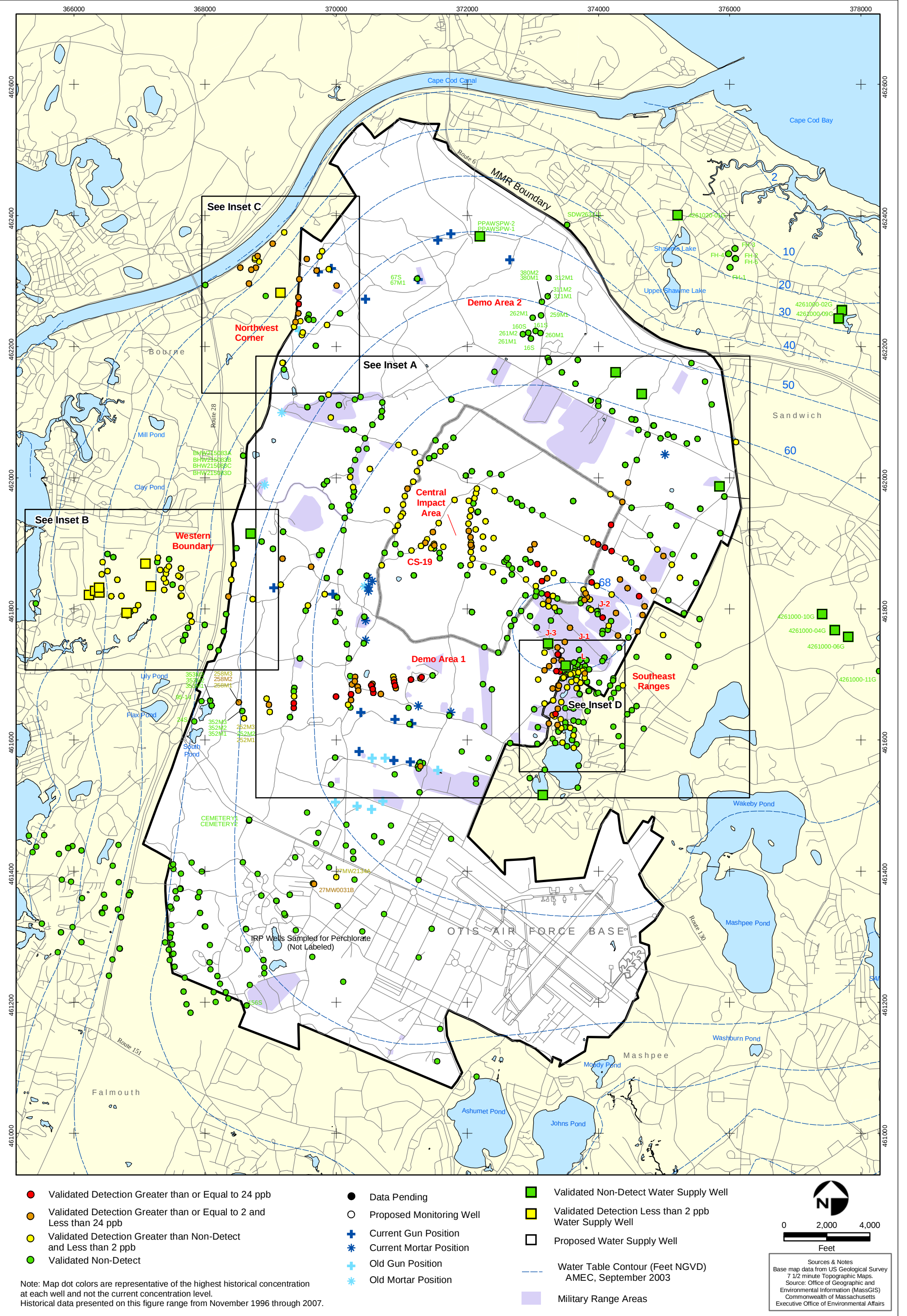
Perchlorate in Groundwater Compared to a 2 ppb Concentration Validated Data as of 8/31/07
