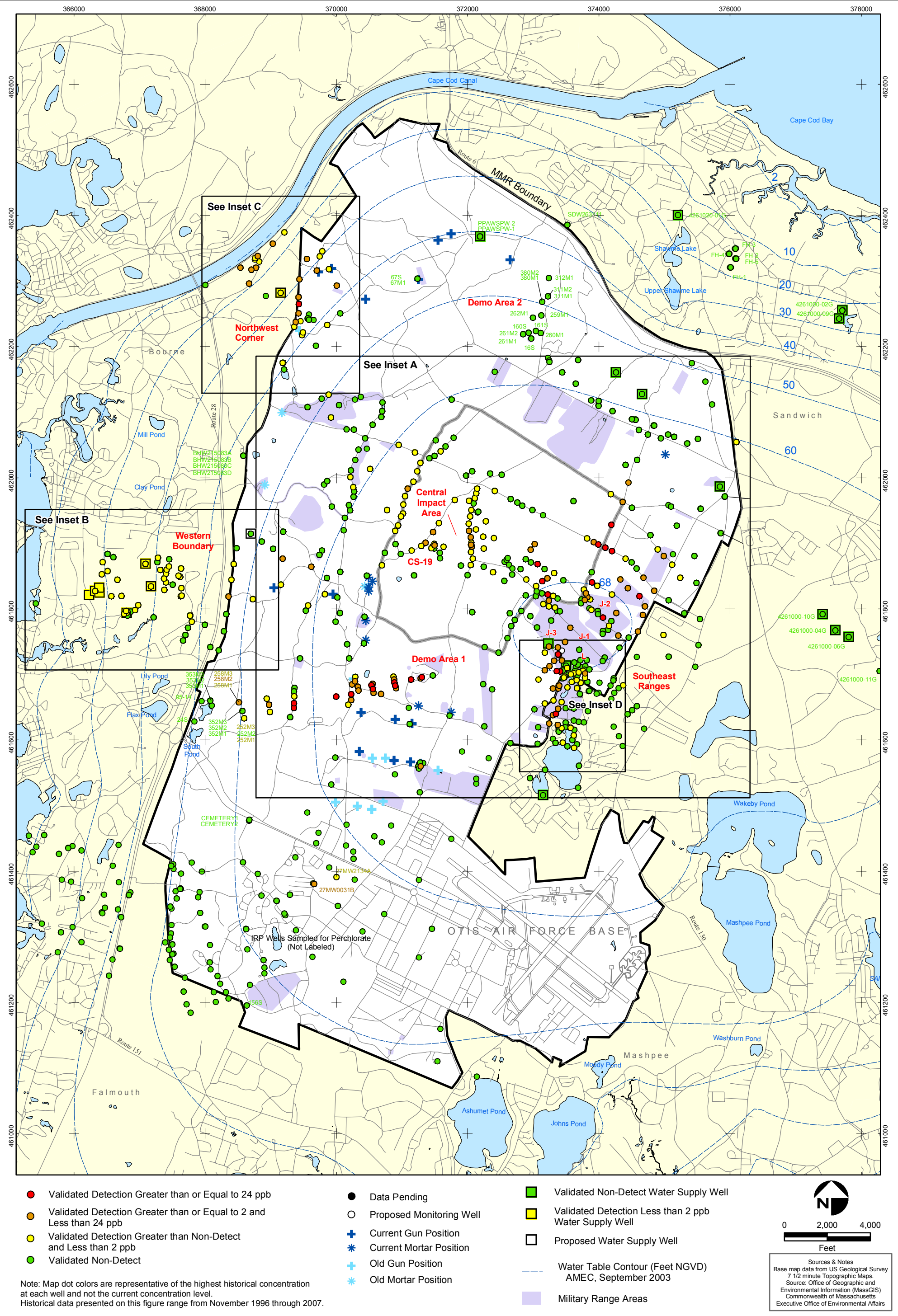
Perchlorate in Groundwater Compared to a 2 ppb Concentration Validated Data as of 6/29/07
