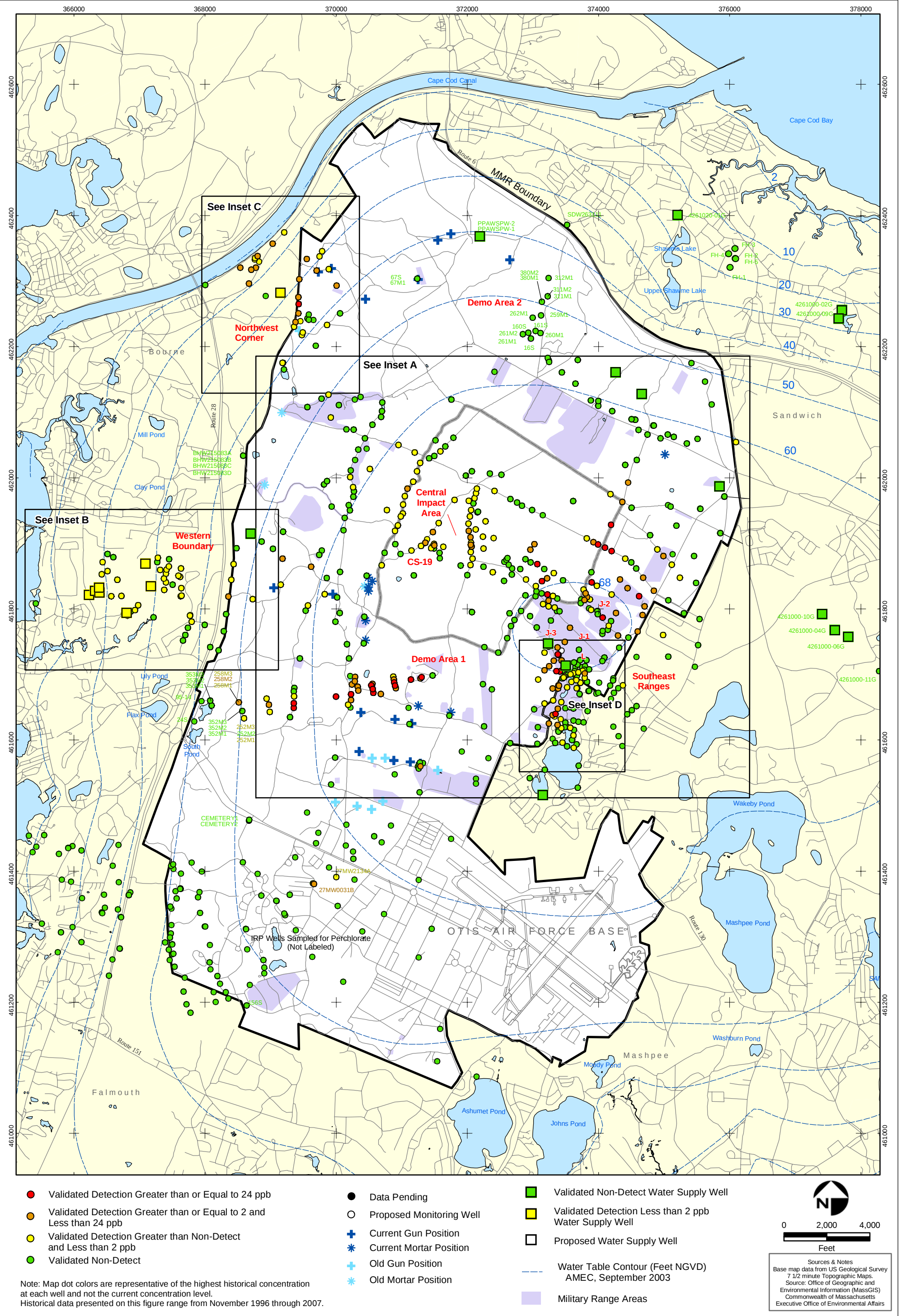
Perchlorate in Groundwater Compared to a 2 ppb Concentration Validated Data as of 9/26/07
