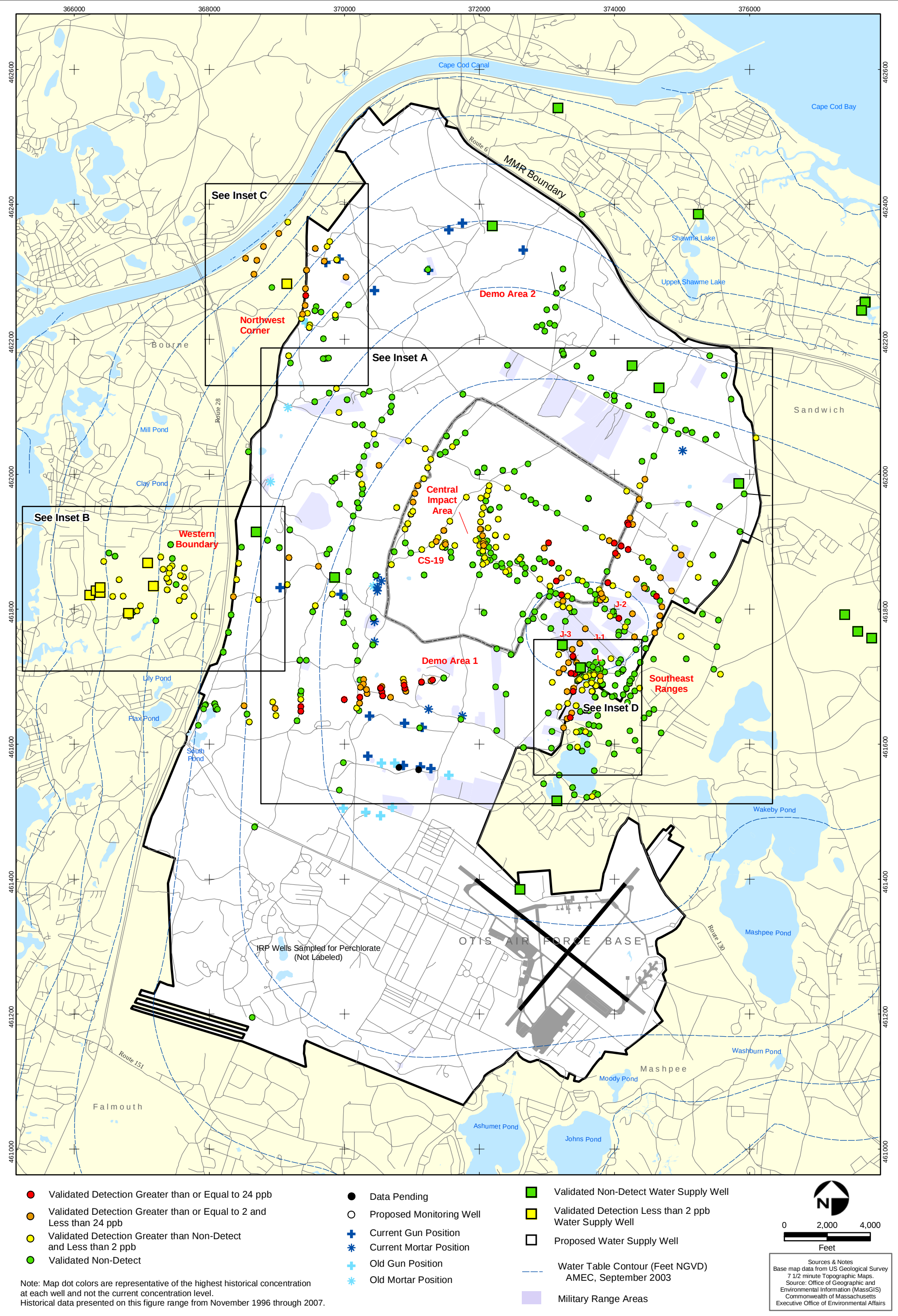
Perchlorate in Groundwater Compared to a 2 ppb Concentration Validated Data as of 12/31/08
